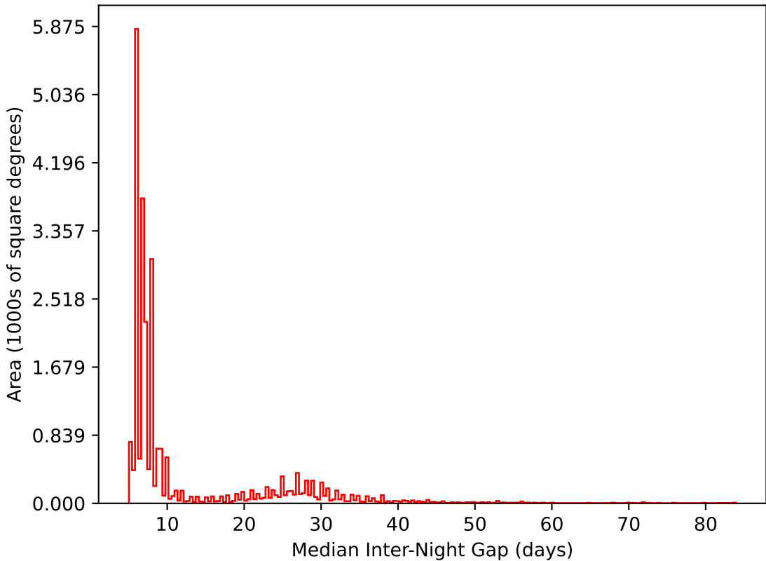
start_date_do90v3.4_10yrs All sky i band: Median Inter-Night Gap
