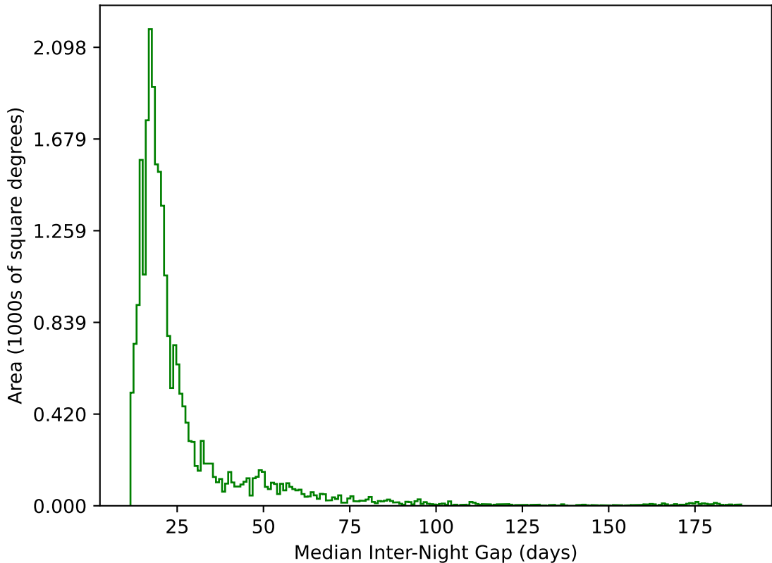
start_date_do90v3.4_10yrs All sky g band: Median Inter-Night Gap
