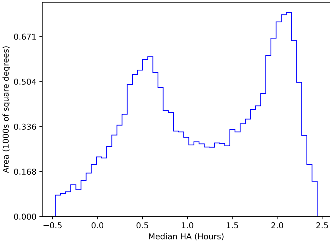
start_date_do90v3.4_10yrs WFD y band: Median HA
