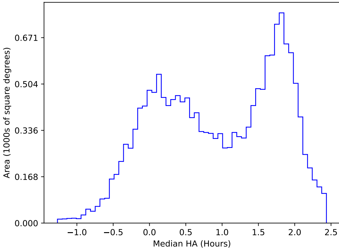
start_date_do90v3.4_10yrs WFD u band: Median HA
