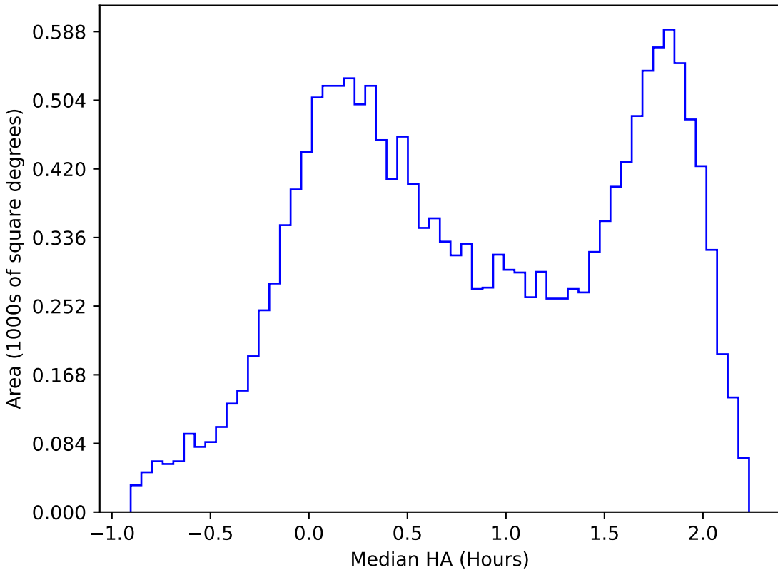
start_date_do90v3.4_10yrs WFD r band: Median HA
