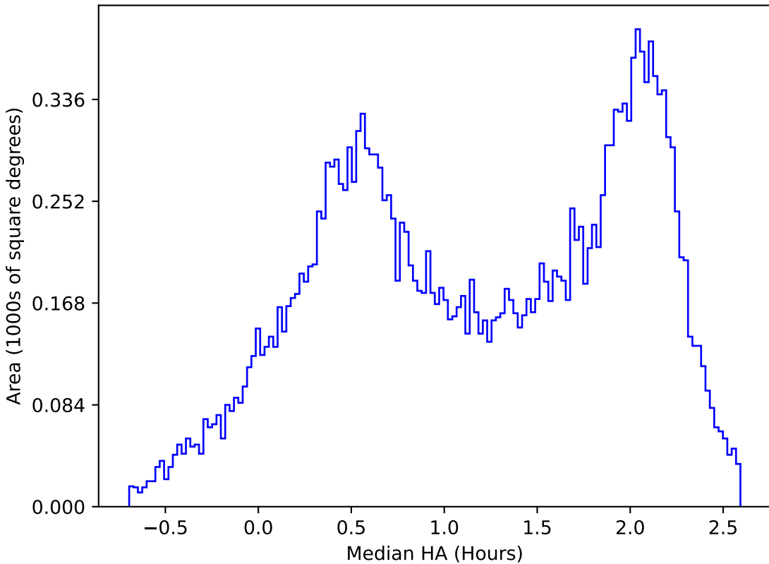
start_date_do90v3.4_10yrs All sky y band: Median HA
