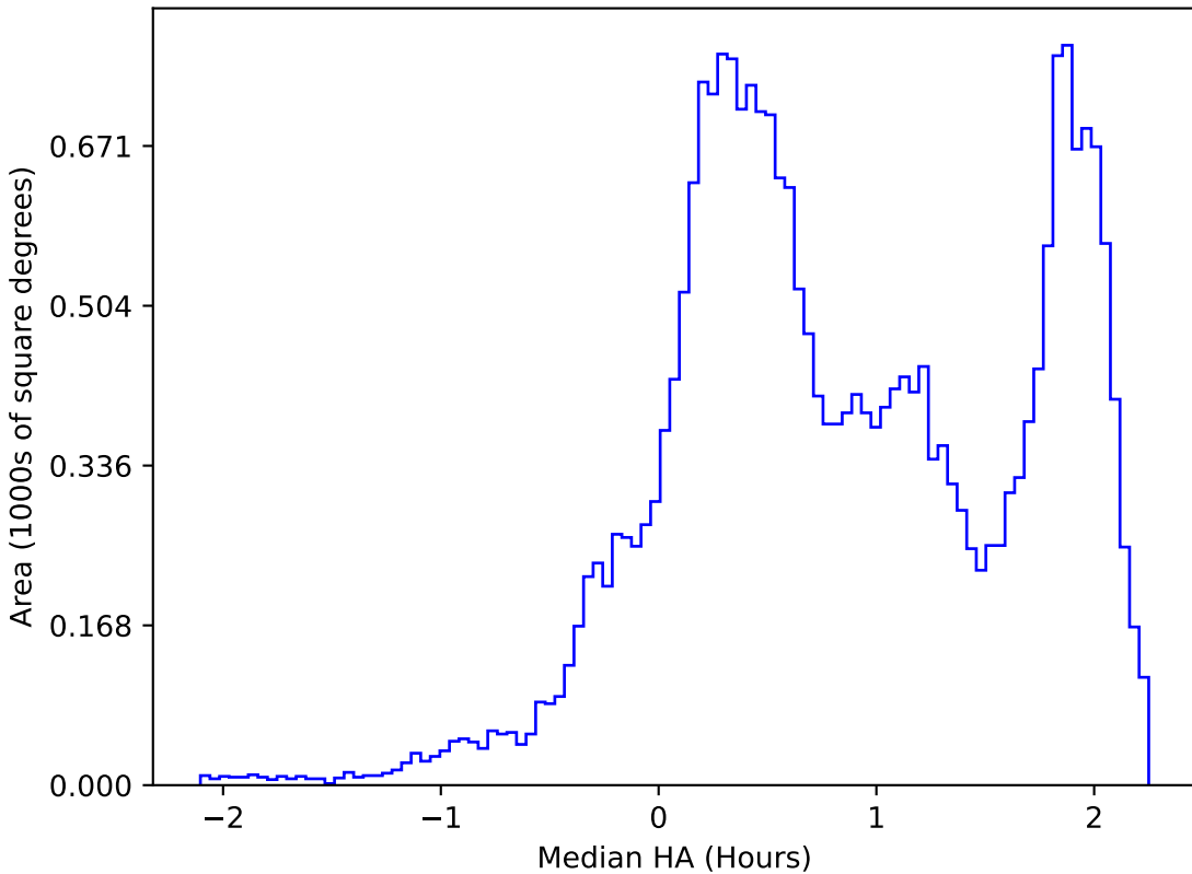
start_date_do90v3.4_10yrs All sky all bands: Median HA
