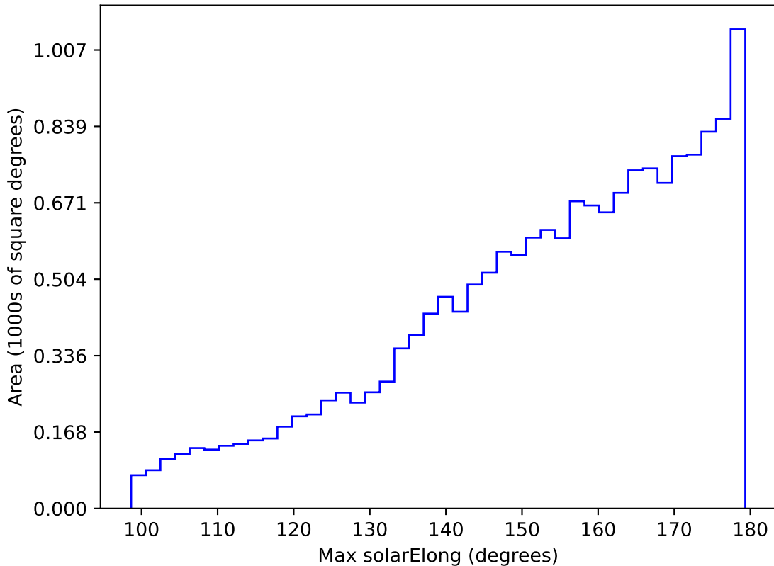
start_date_do90v3.4_10yrs WFD z band: Max solarElong
