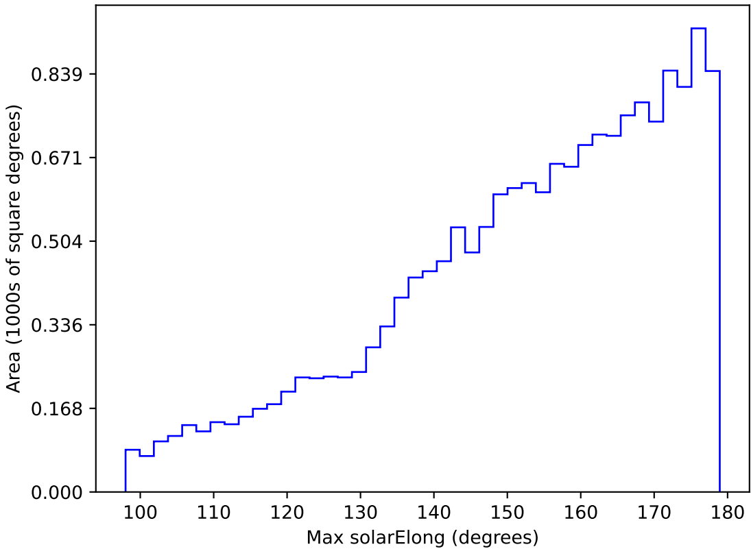
start_date_do90v3.4_10yrs WFD u band: Max solarElong
