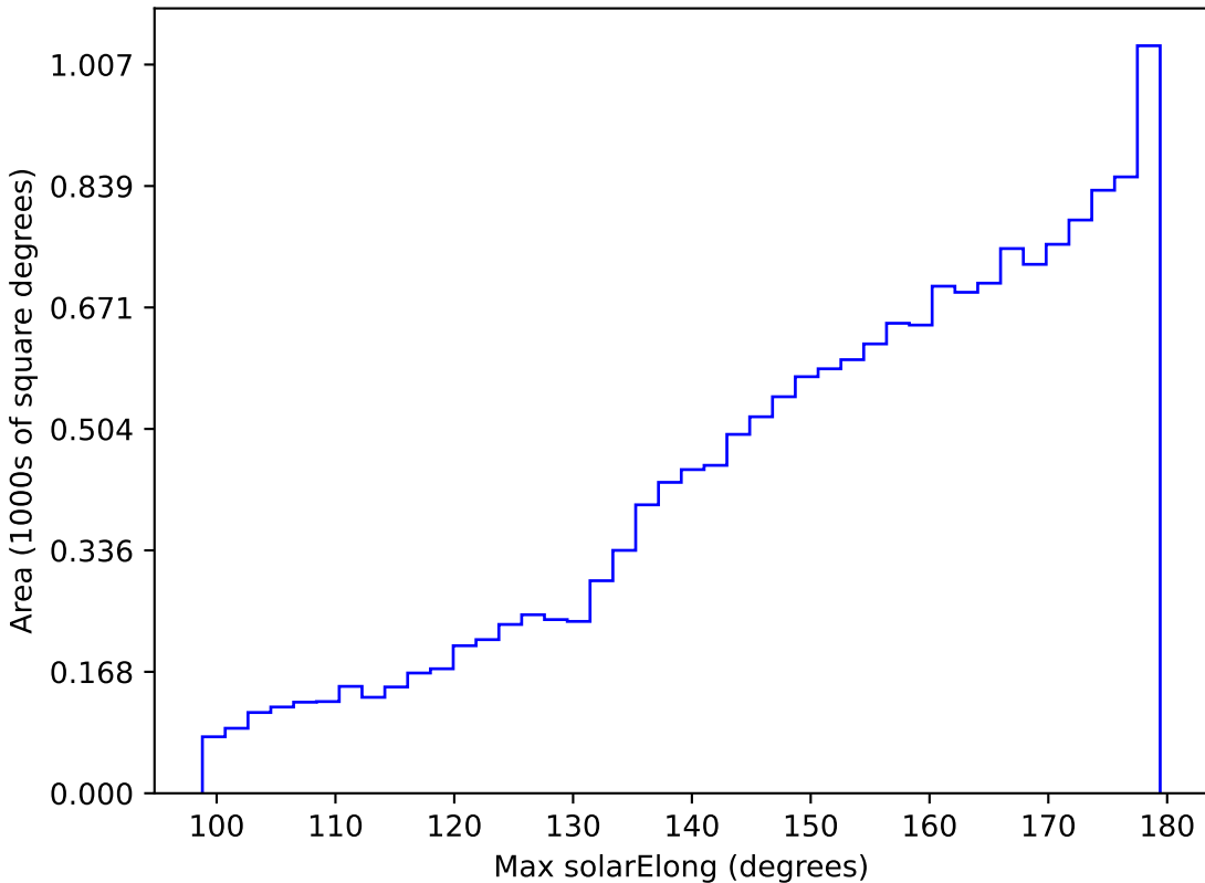
start_date_do90v3.4_10yrs WFD r band: Max solarElong
