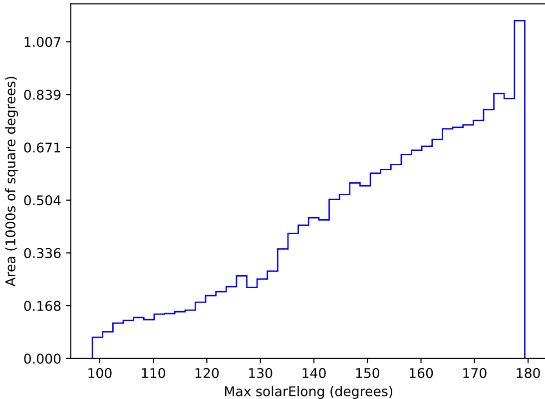
start_date_do90v3.4_10yrs WFD i band: Max solarElong
