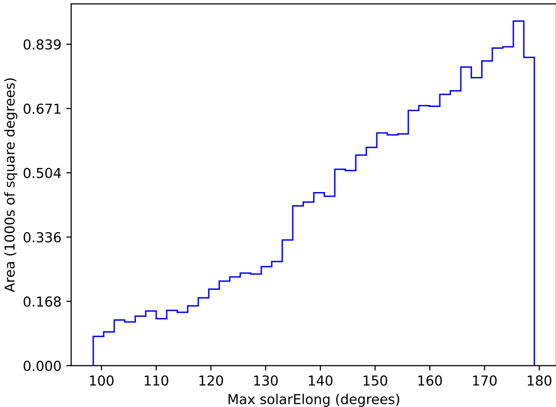
start_date_do90v3.4_10yrs WFD g band: Max solarElong
