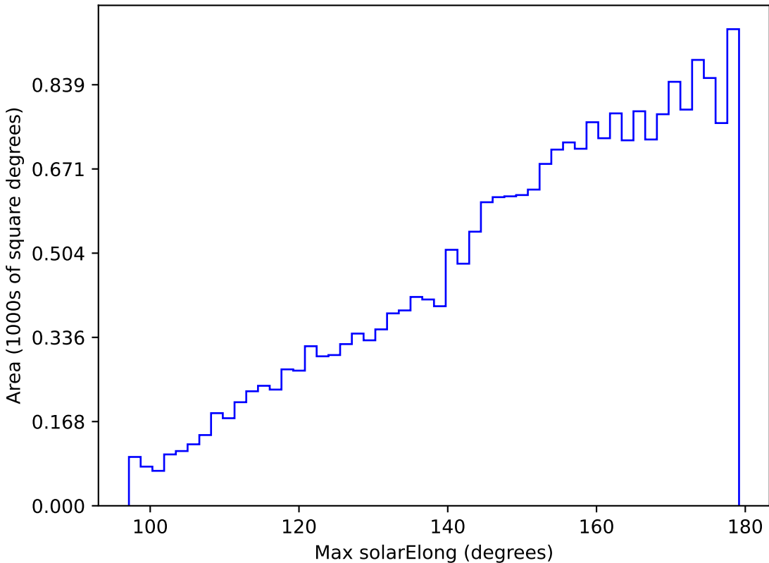
start_date_do90v3.4_10yrs All sky y band: Max solarElong
