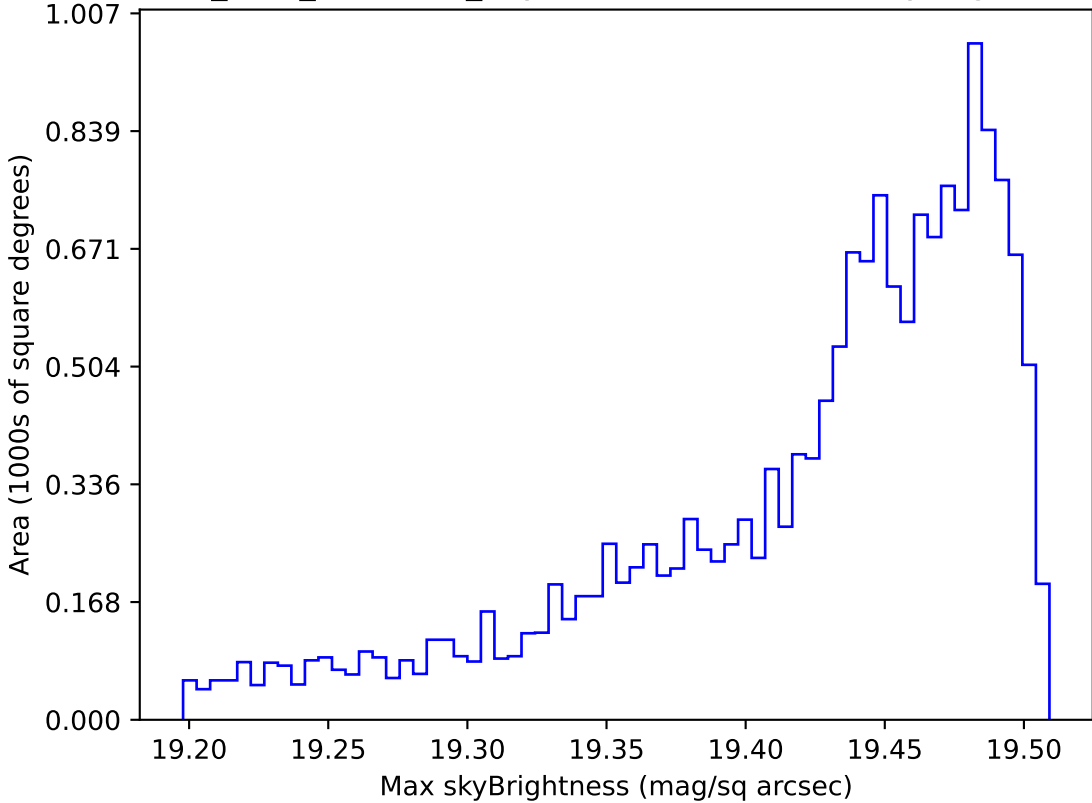
start_date_do90v3.4_10yrs WFD z band: Max skyBrightness
