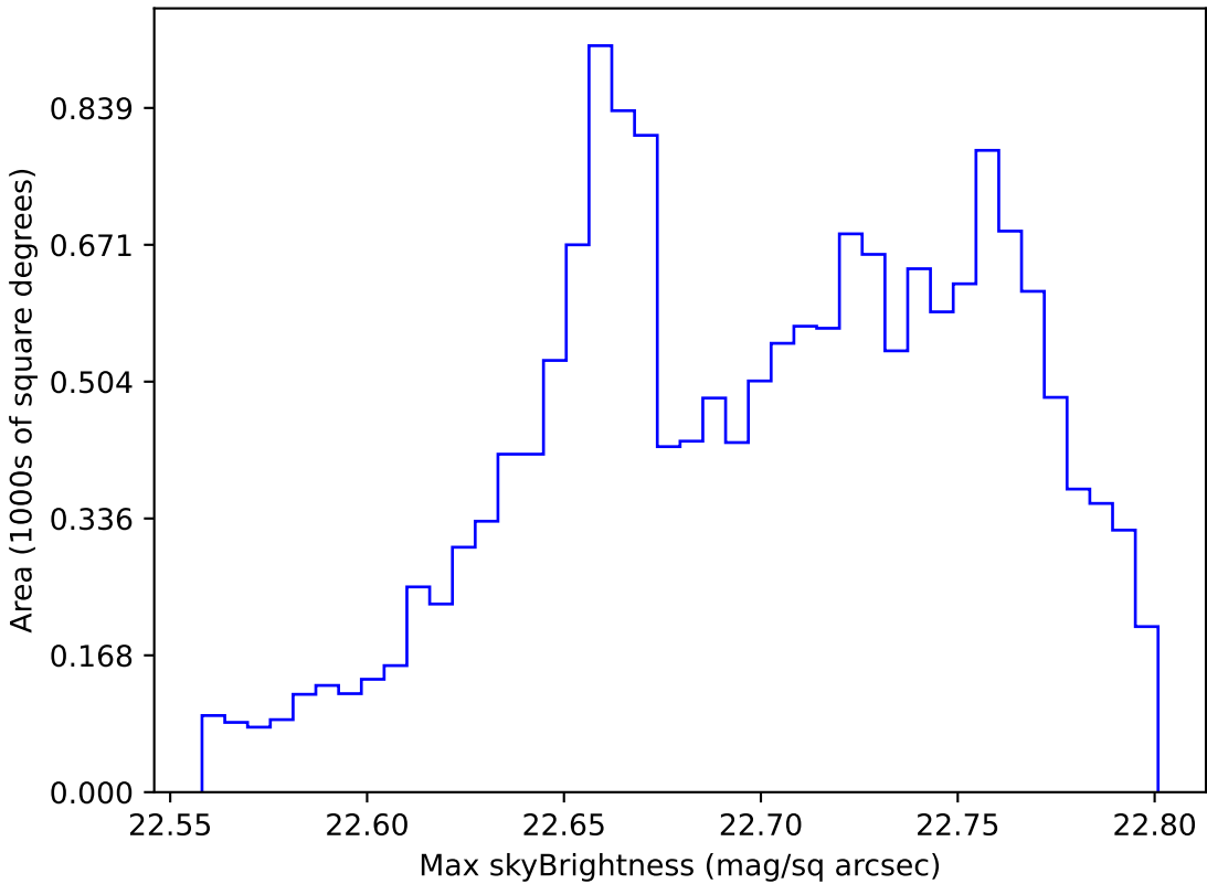
start_date_do90v3.4_10yrs WFD u band: Max skyBrightness
