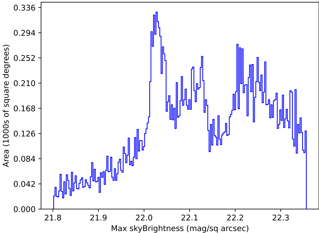
start_date_do90v3.4_10yrs All sky g band: Max skyBrightness
