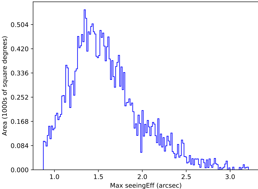
start_date_do90v3.4_10yrs Yr 1 g band: Max seeingEff
