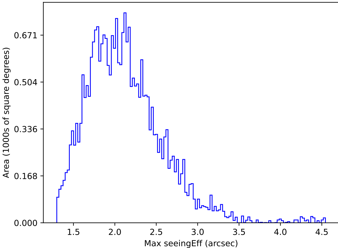
start_date_do90v3.4_10yrs Yr 1 all bands: Max seeingEff
