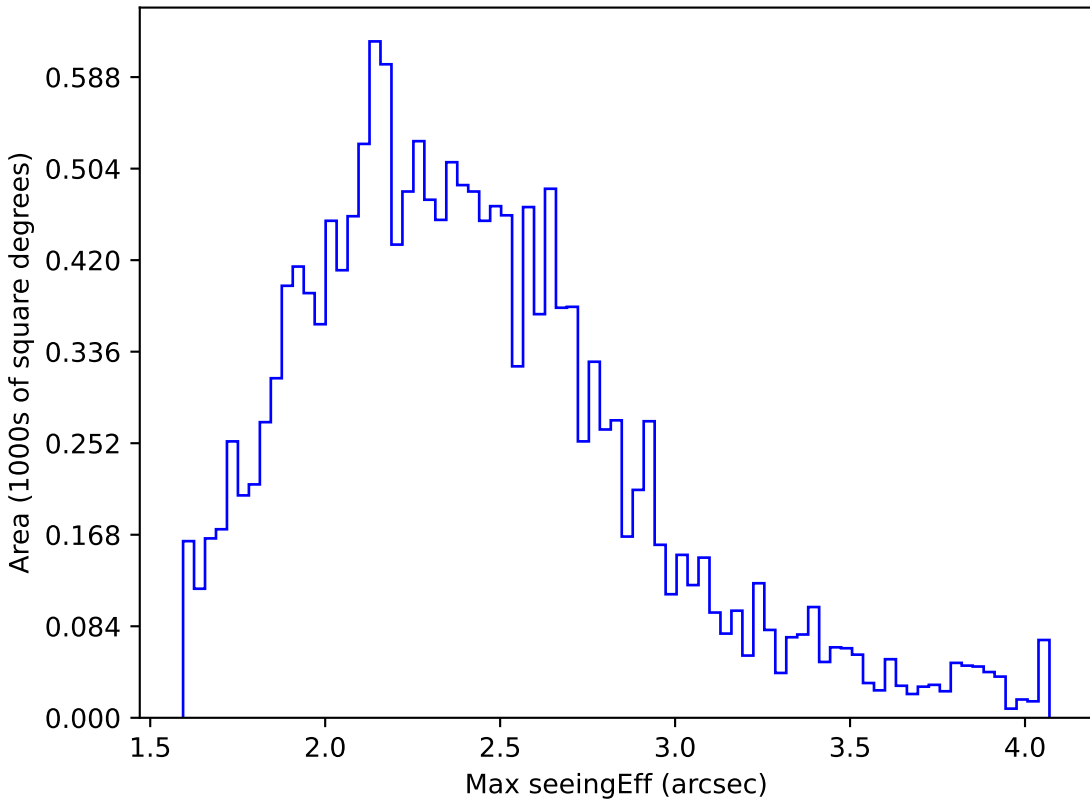
start_date_do90v3.4_10yrs WFD y band: Max seeingEff
