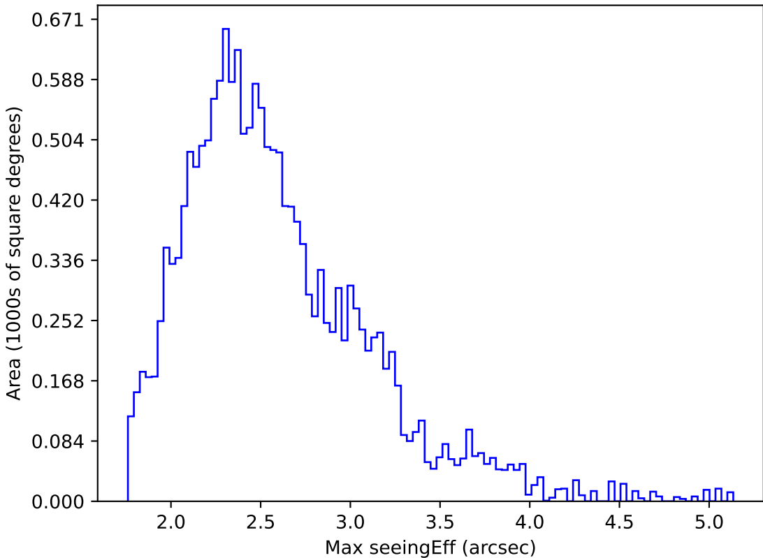
start_date_do90v3.4_10yrs WFD u band: Max seeingEff
