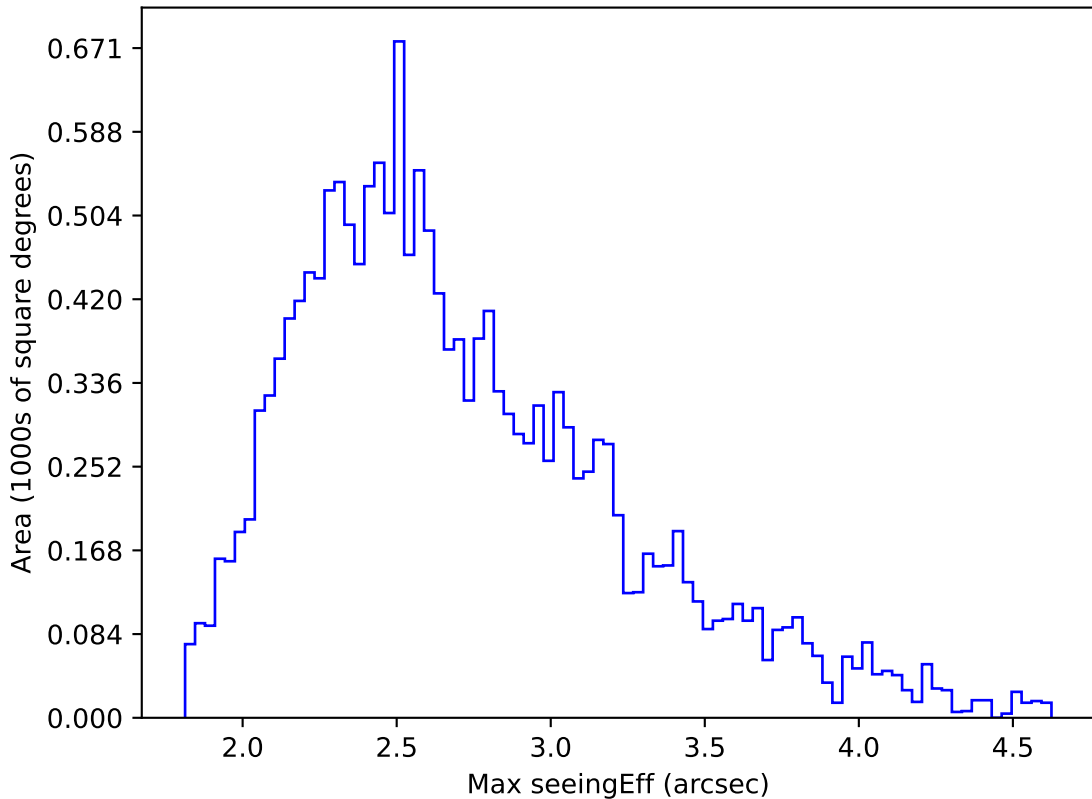
start_date_do90v3.4_10yrs WFD r band: Max seeingEff
