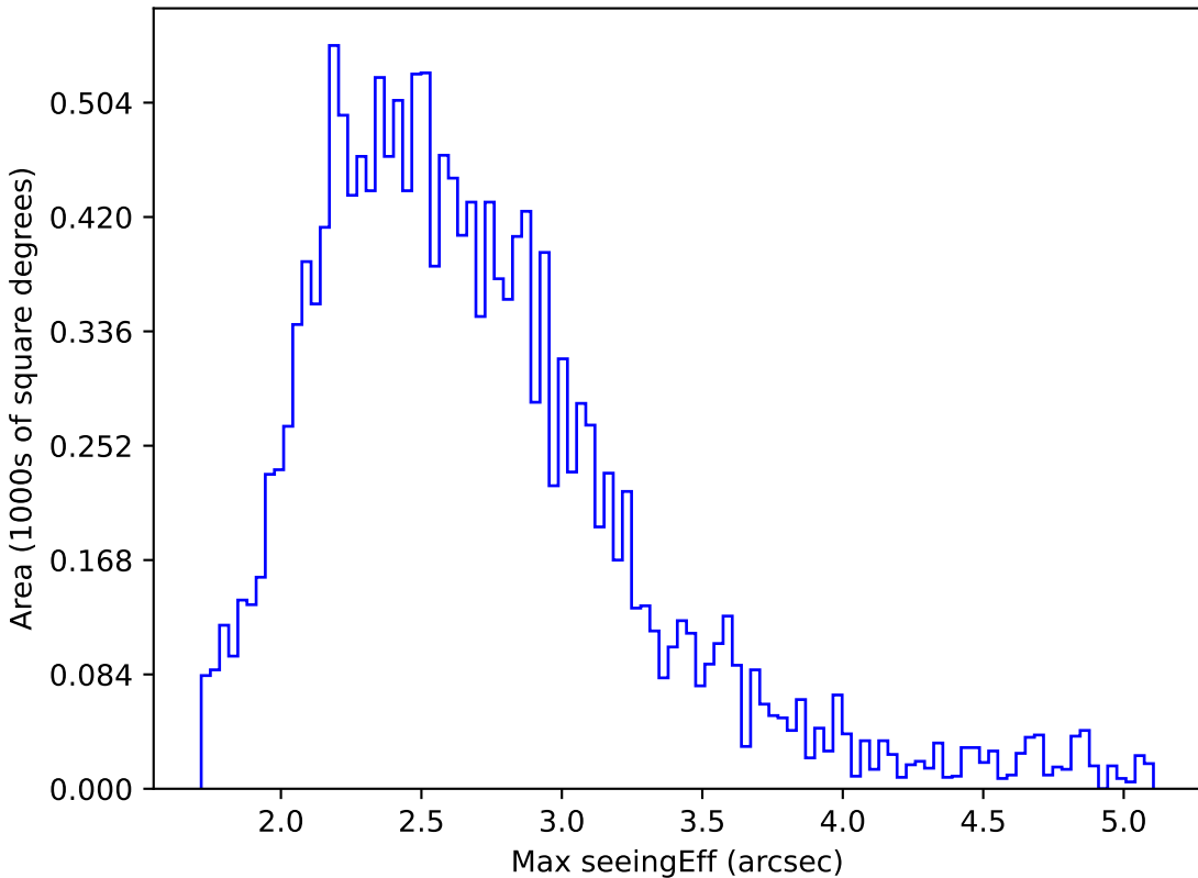
start_date_do90v3.4_10yrs WFD i band: Max seeingEff
