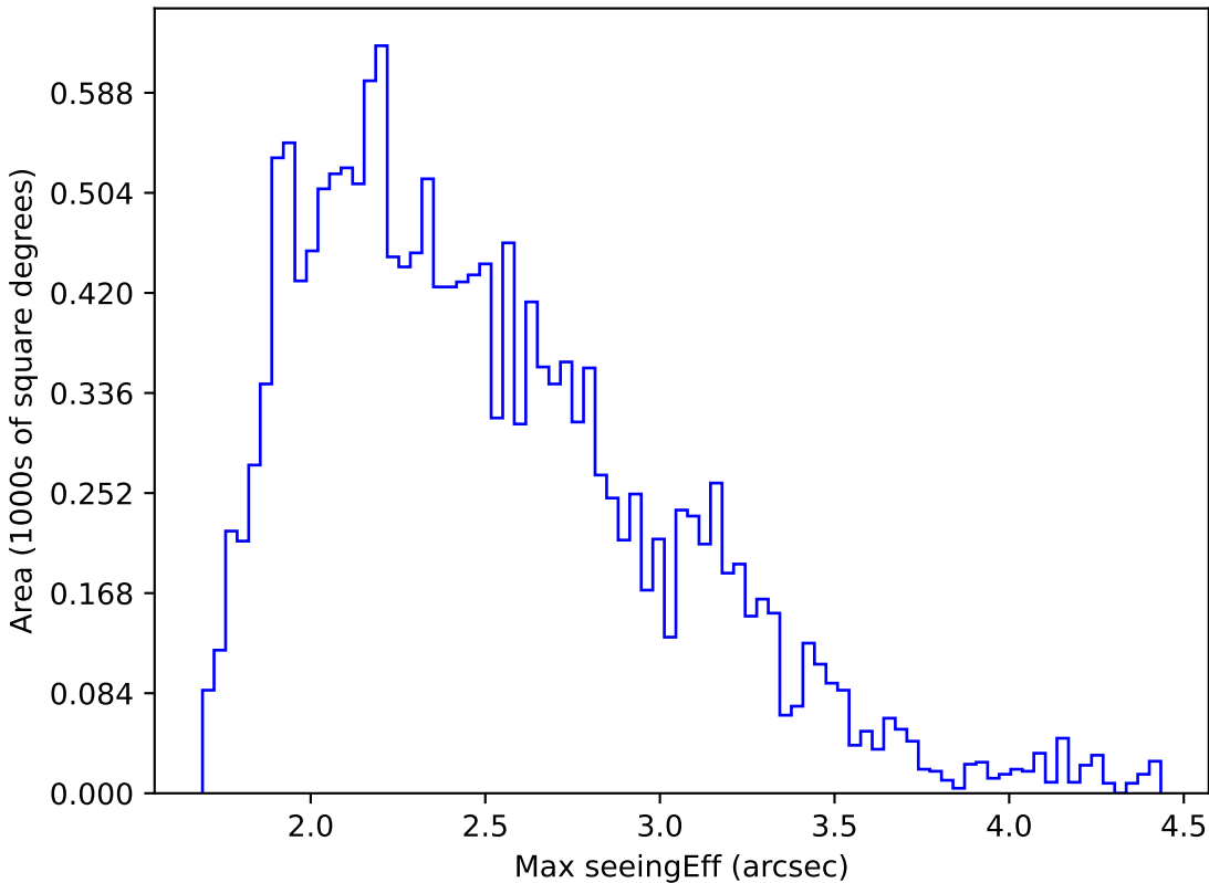
start_date_do90v3.4_10yrs WFD g band: Max seeingEff
