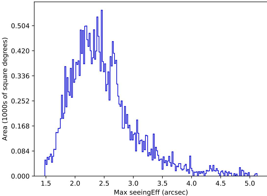
start_date_do90v3.4_10yrs All sky z band: Max seeingEff
