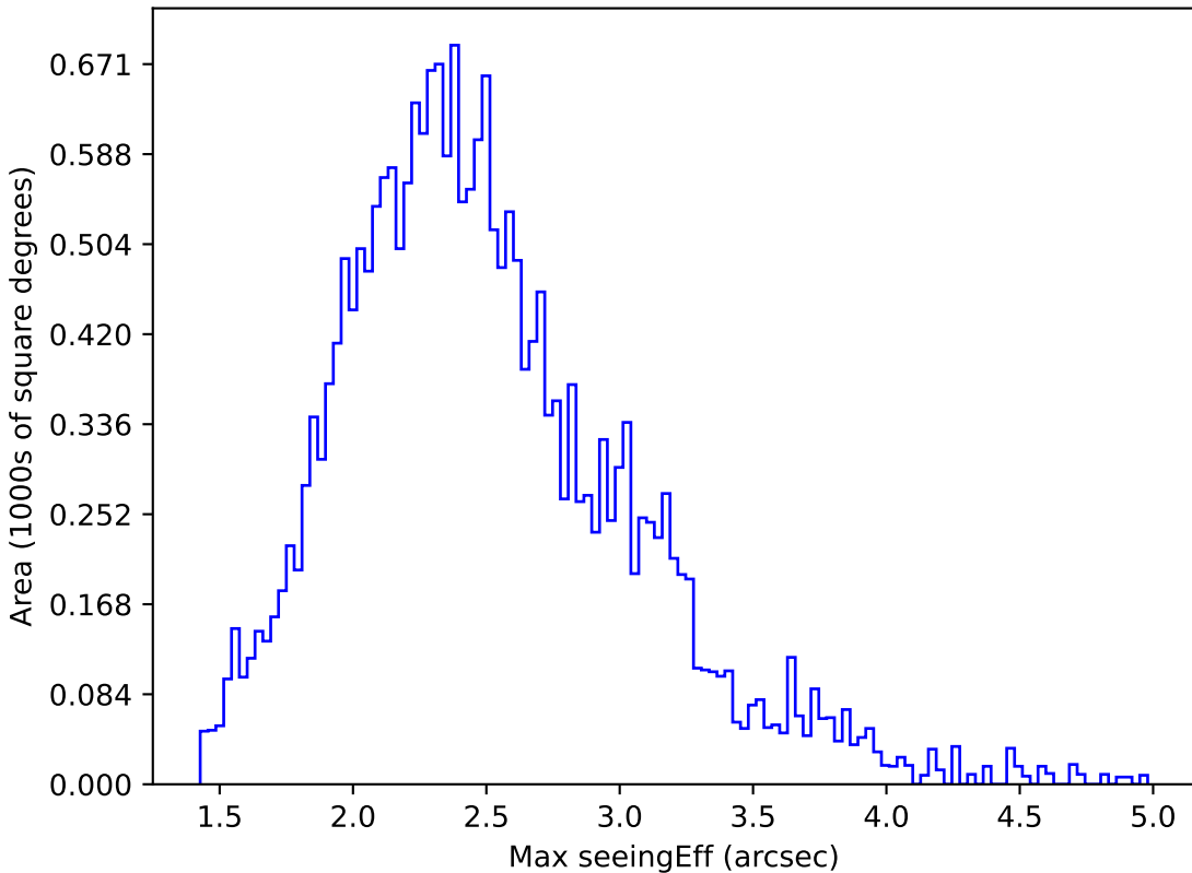
start_date_do90v3.4_10yrs All sky u band: Max seeingEff
