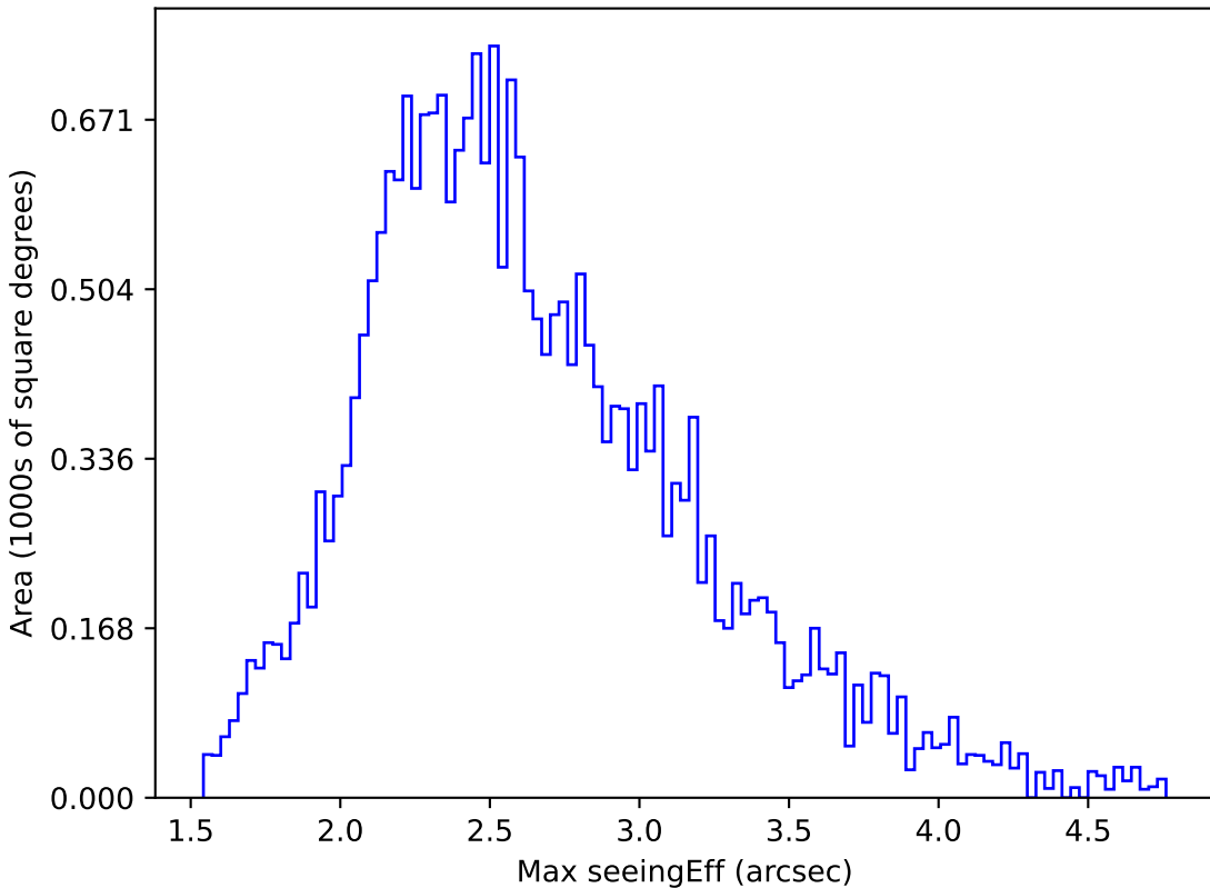
start_date_do90v3.4_10yrs All sky r band: Max seeingEff
