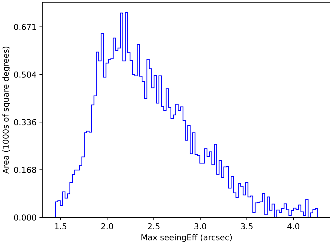
start_date_do90v3.4_10yrs All sky g band: Max seeingEff
