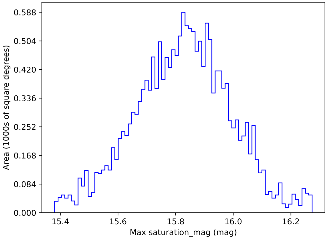
start_date_do90v3.4_10yrs WFD all bands: Max saturation_mag
