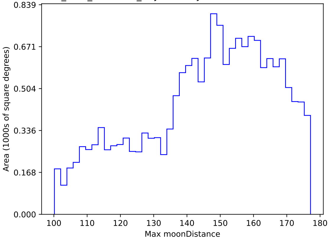
start_date_do90v3.4_10yrs WFD y band: Max moonDistance
