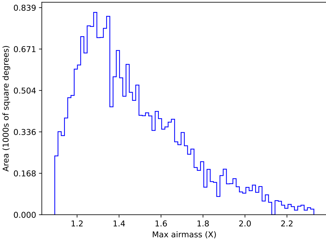
start_date_do90v3.4_10yrs Yr 1 u band: Max airmass
