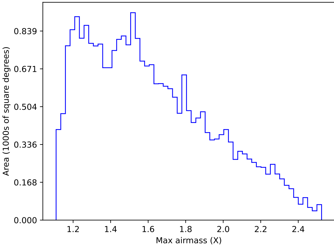
start_date_do90v3.4_10yrs Yr 1 g band: Max airmass
