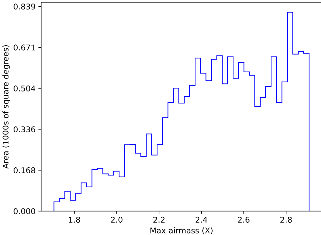
start_date_do90v3.4_10yrs WFD i band: Max airmass
