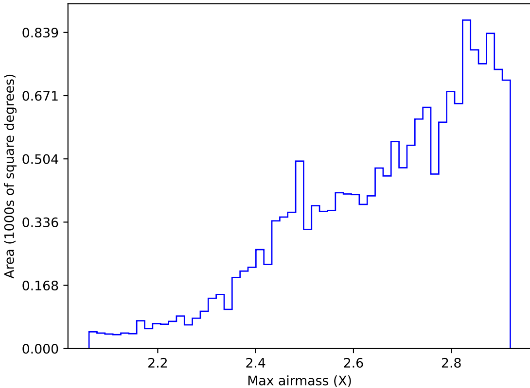
start_date_do90v3.4_10yrs WFD all bands: Max airmass
