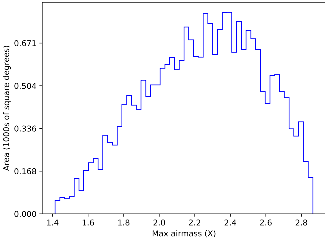
start_date_do90v3.4_10yrs All sky y band: Max airmass
