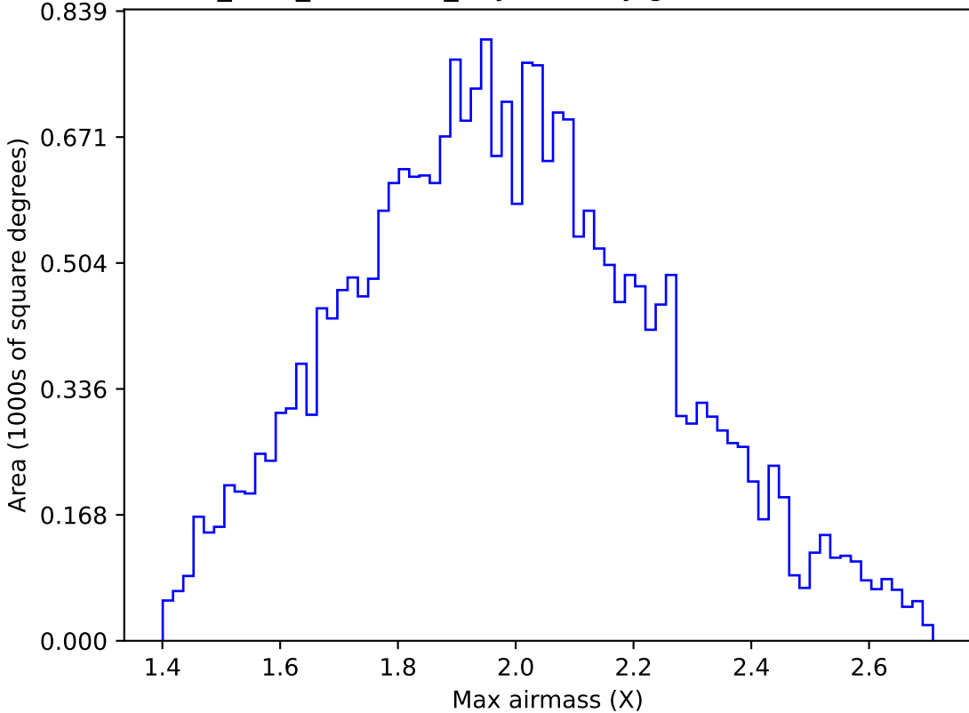
start_date_do90v3.4_10yrs All sky g band: Max airmass
