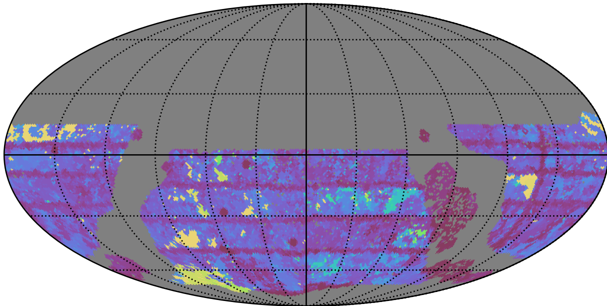
start_date_do90v3.4_10yrs WFD r band: Max Inter-Night Gap
