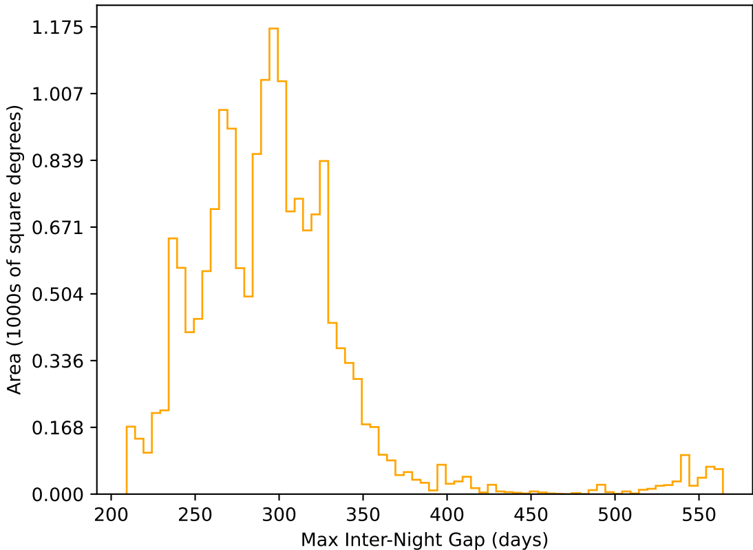
start_date_do90v3.4_10yrs WFD r band: Max Inter-Night Gap
