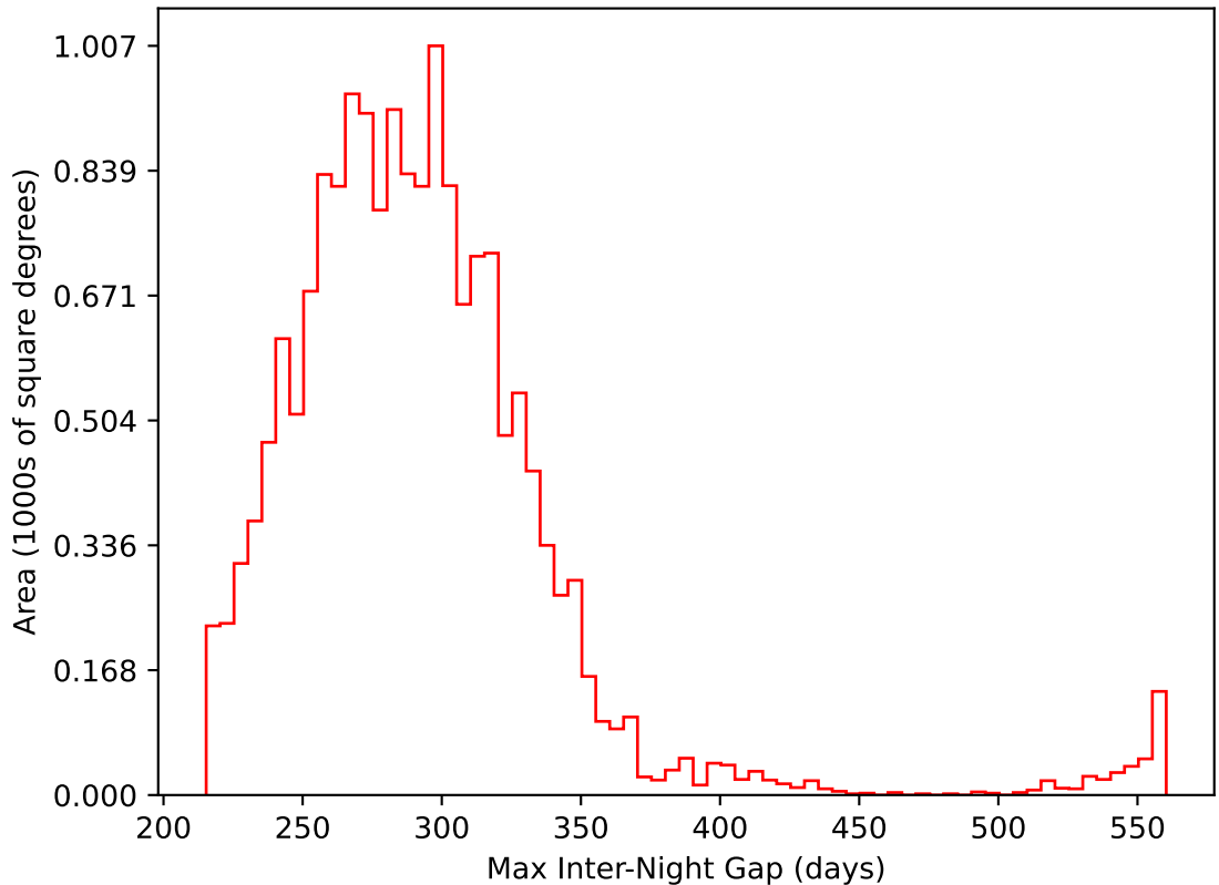
start_date_do90v3.4_10yrs WFD i band: Max Inter-Night Gap
