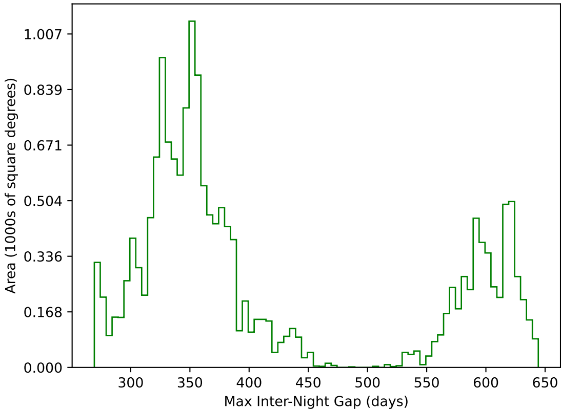
start_date_do90v3.4_10yrs WFD g band: Max Inter-Night Gap
