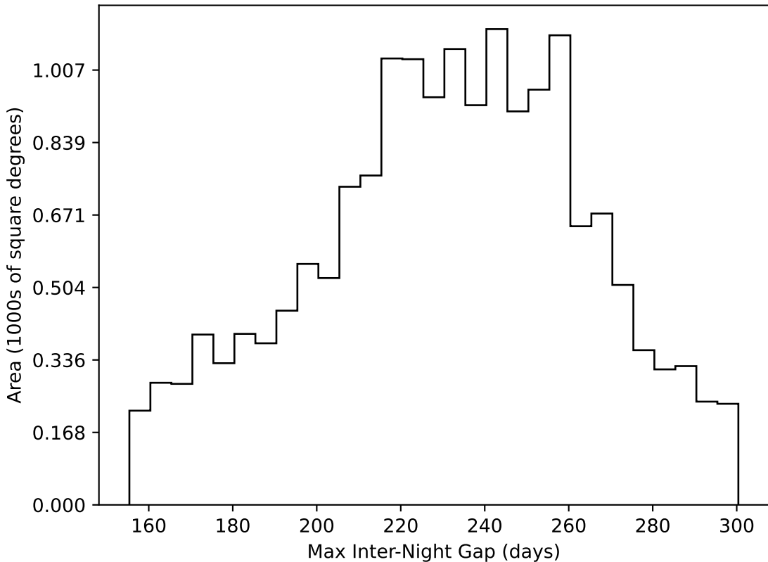
start_date_do90v3.4_10yrs WFD all bands: Max Inter-Night Gap
