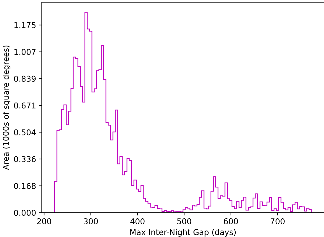
start_date_do90v3.4_10yrs All sky z band: Max Inter-Night Gap
