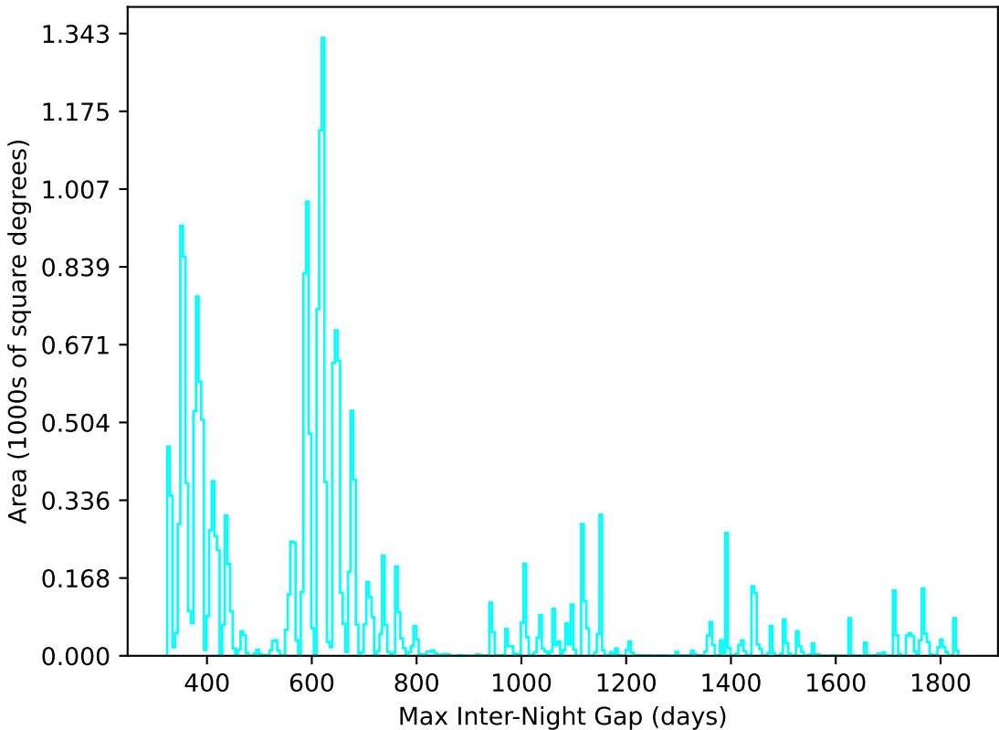
start_date_do90v3.4_10yrs All sky u band: Max Inter-Night Gap
