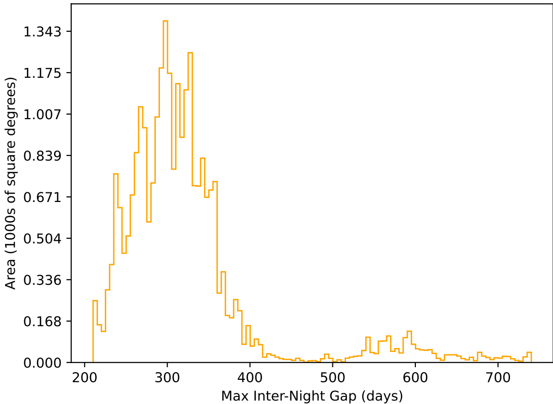
start_date_do90v3.4_10yrs All sky r band: Max Inter-Night Gap
