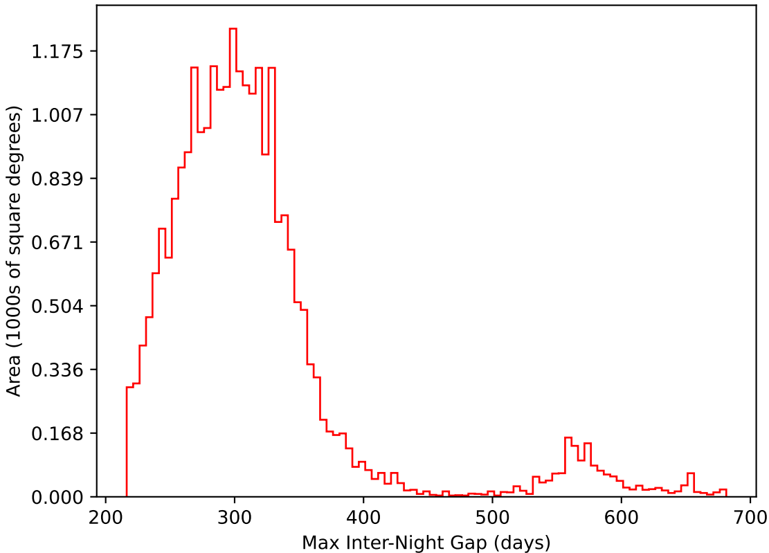
start_date_do90v3.4_10yrs All sky i band: Max Inter-Night Gap
