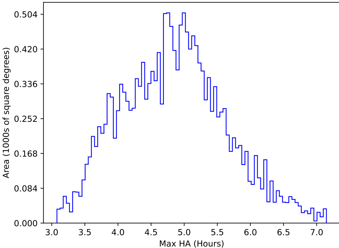
start_date_do90v3.4_10yrs WFD z band: Max HA
