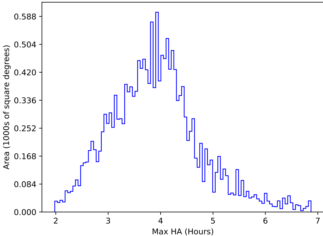
start_date_do90v3.4_10yrs WFD u band: Max HA
