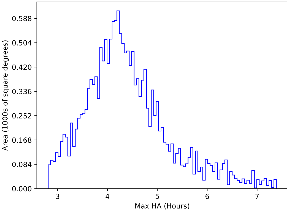
start_date_do90v3.4_10yrs WFD r band: Max HA
