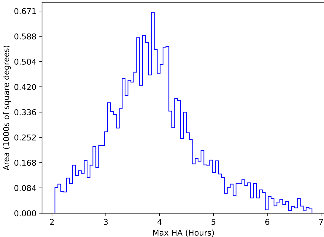
start_date_do90v3.4_10yrs WFD g band: Max HA
