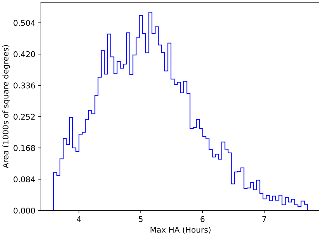
start_date_do90v3.4_10yrs WFD all bands: Max HA
