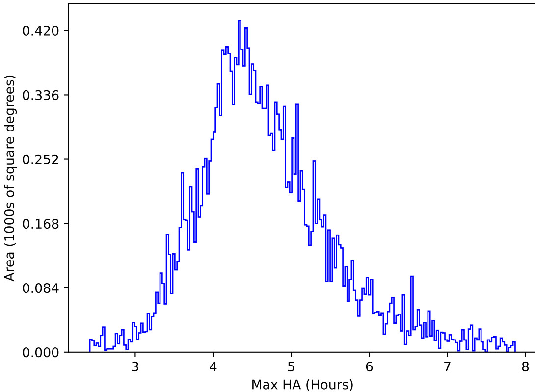
start_date_do90v3.4_10yrs All sky y band: Max HA
